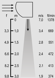
Air Flow
